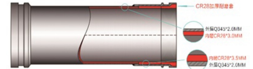
CR28加长法兰双层管 CR 28 LENGTHEN THE FLANGE DOUBLE LAYER PIPE
